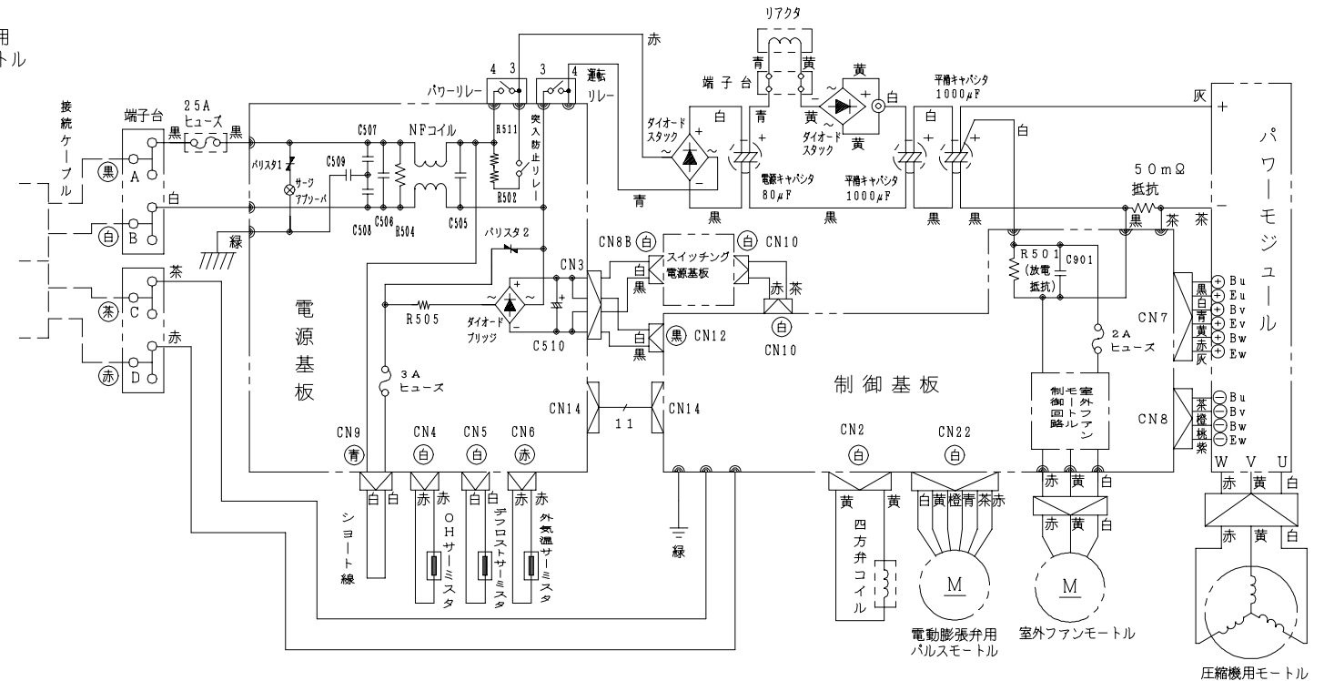
RAC-40SKX2配線図
